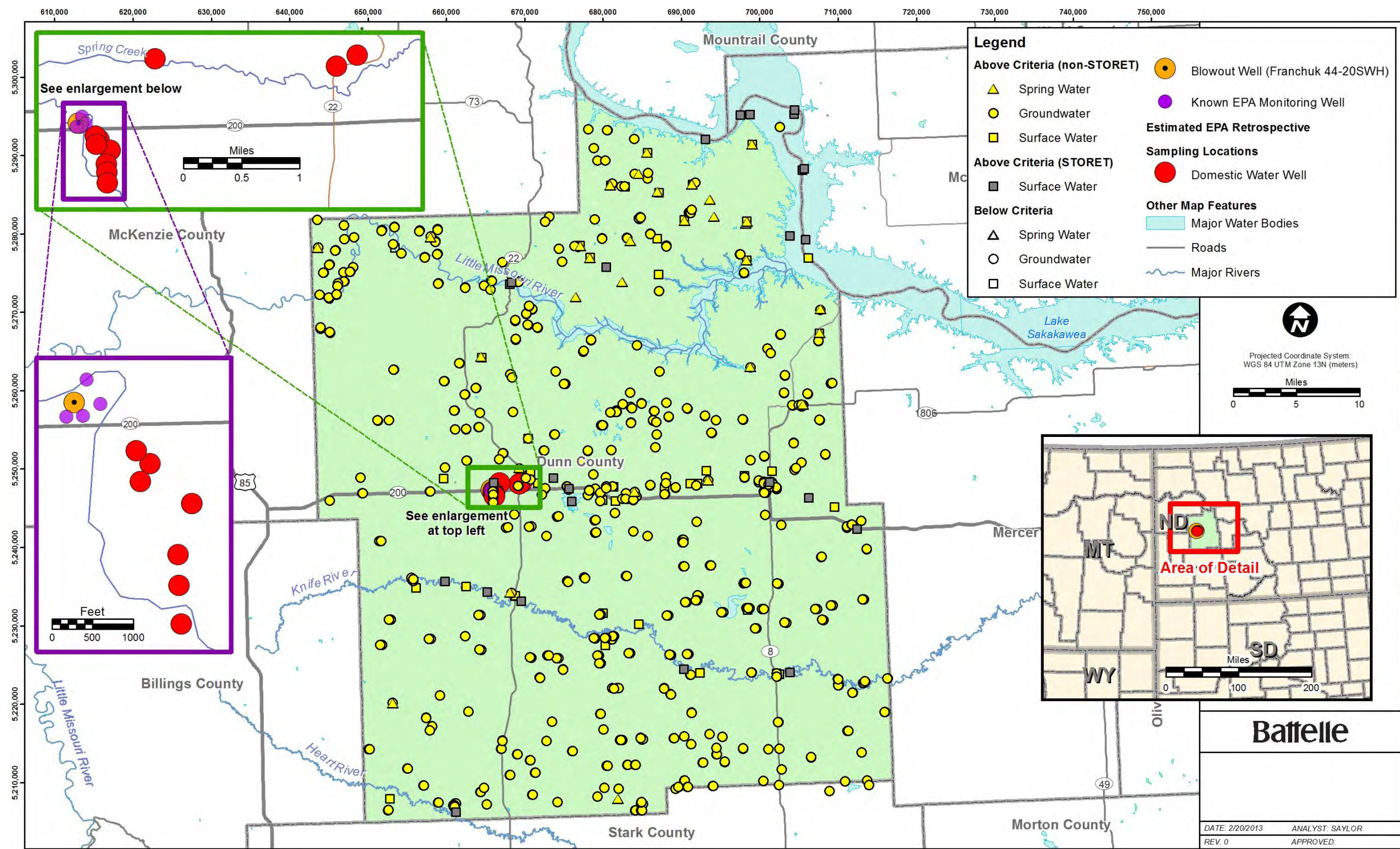
Figure 3-6. Groundwater, Surface Water, and Spring Detections above Screening Criteria, Dunn County, ND
