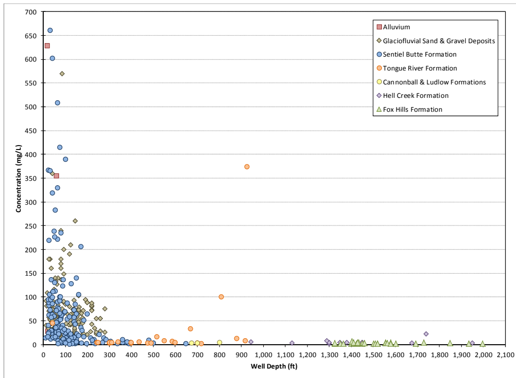
Figure 3-10a. Correlation of Depth and Formation with Concentrations of Calcium
