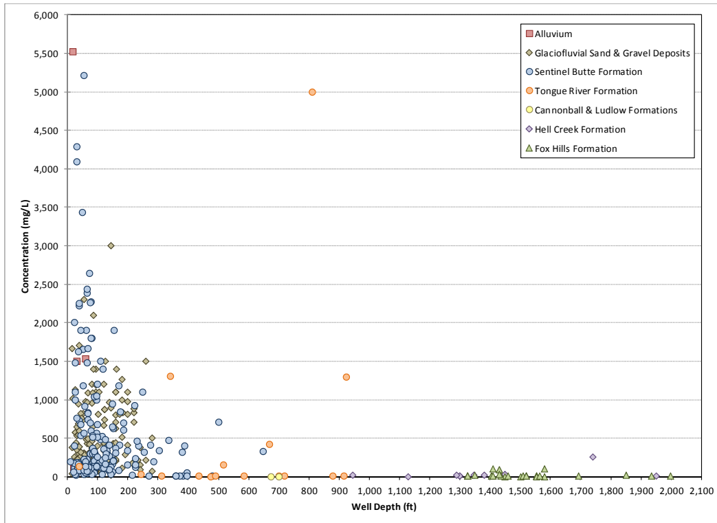
Figure 3-10e. Correlation of Depth and Formation with Concentrations of Sulfate
