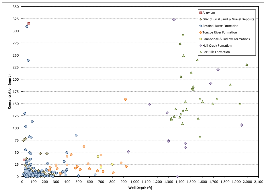
Figure 3-10b. Correlation of Depth and Formation with Concentrations of Chloride
