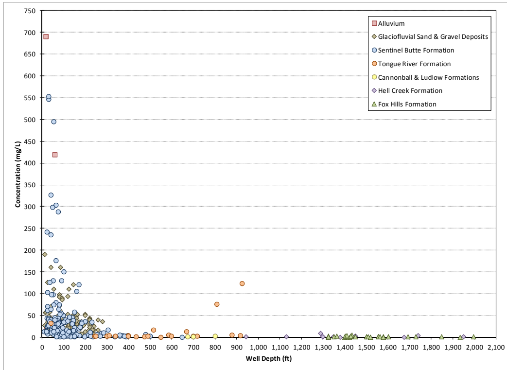
Figure 3-10c. Correlation of Depth and Formation with Concentrations of Magnesium
