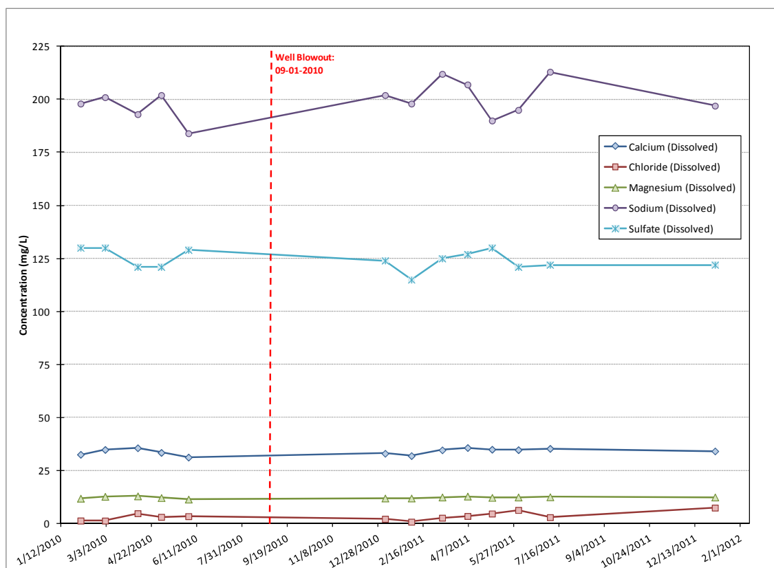
Figure 3-8. Time-Series Concentrations for Calcium, Chloride, Magnesium, Sodium, and Sulfate in Groundwater in Well 126374
