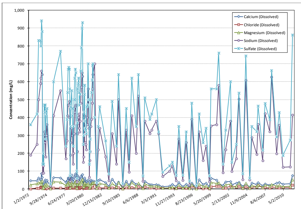
Figure 3-12b. Surface Water Quality Measured at USGS Station 06339100
