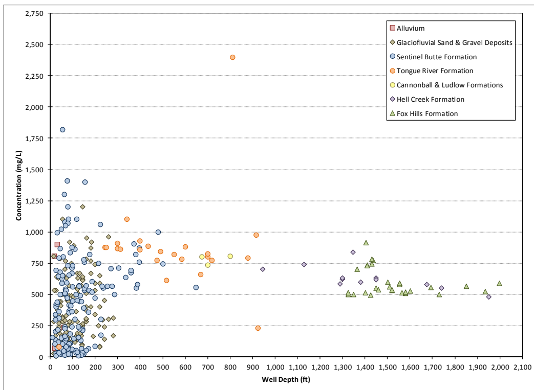
Figure 3-10d. Correlation of Depth and Formation with Concentrations of Sodium
