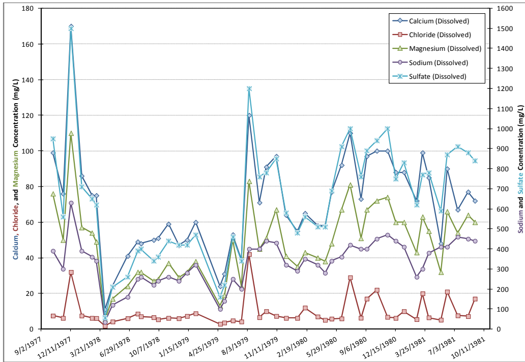
Figure 3-12a. Surface Water Quality Measured at USGS Station 06339800
