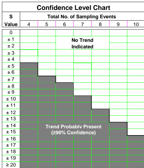
Figure F-1 Worksheet for Concentration Trend Analysis using the Mann-Kendall Test (From Wiedemeier et al., 1999)
