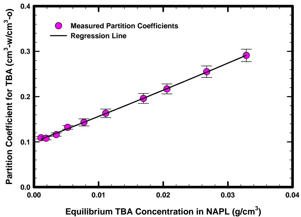
Figure 9a-b. Effect of higher concentrations on partition coefficients for TBA partitioning between a NAPL mixture and an aqueous phase at 24 °C. Partition coefficients are plotted vs. equilibrium aqueous concentration (a) and NAPL concentration (b).
