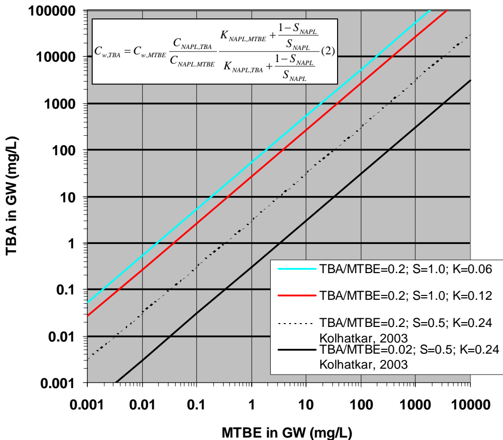
Figures 8a-b. Calculated concentrations of TBA in water vs. MTBE concentrations in ground water near a NAPL source. Calculations are based on Equation 2 for various values of K_{NAPL} for TBA and ratios of concentrations of TBA to MTBE in the NAPL. Figure 8a is reproduced from Kolhatkar, 2003. Curves from 8a are also shown in 8b. Note S_{NAPL}=0.5 corresponds to V_{NAPL}/V_w=1 ; S_{NAPL}=1 corresponds to V_{NAPL}/V_w=\infty .
