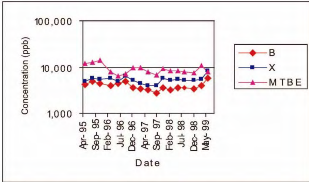
Figure 4-3 Concentrations of MtBE, Benzene, and Xylene in Groundwater in a Monitoring Well with a NAPL Source
