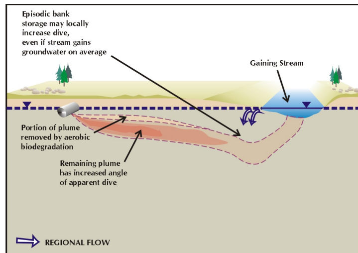
Figure 4. Example of a Diving Plume Near a Gaining Stream
