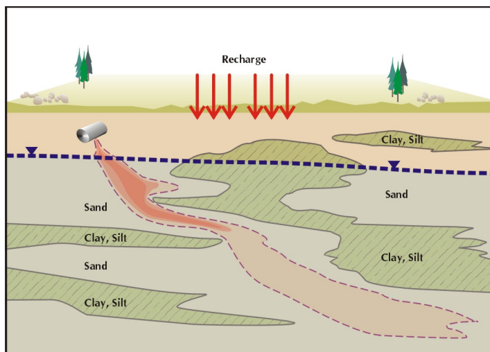
Figure 5. Example of a Diving Plume due to Stratigraphic Controls
