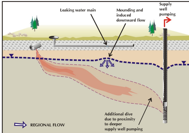
Figure 3. Example of a Diving Plume Along Leaking Water Main and Supply Wells
