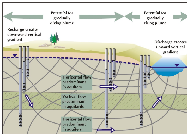
Figure 2. Expected groundwater flow conditions within a watershed
