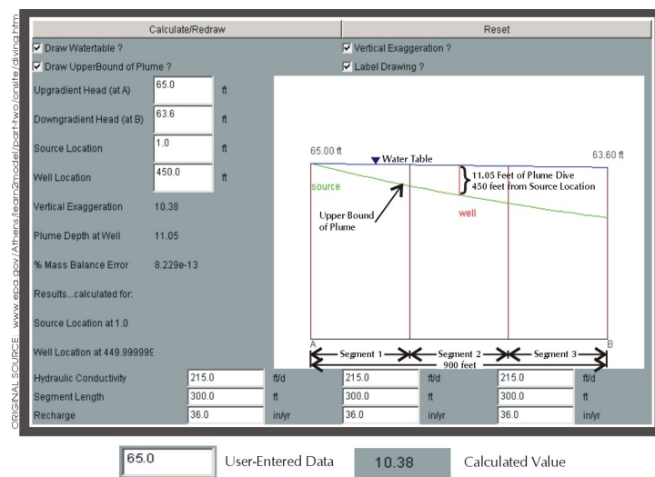
Figure 6. EPA Plume Dive Calculator
