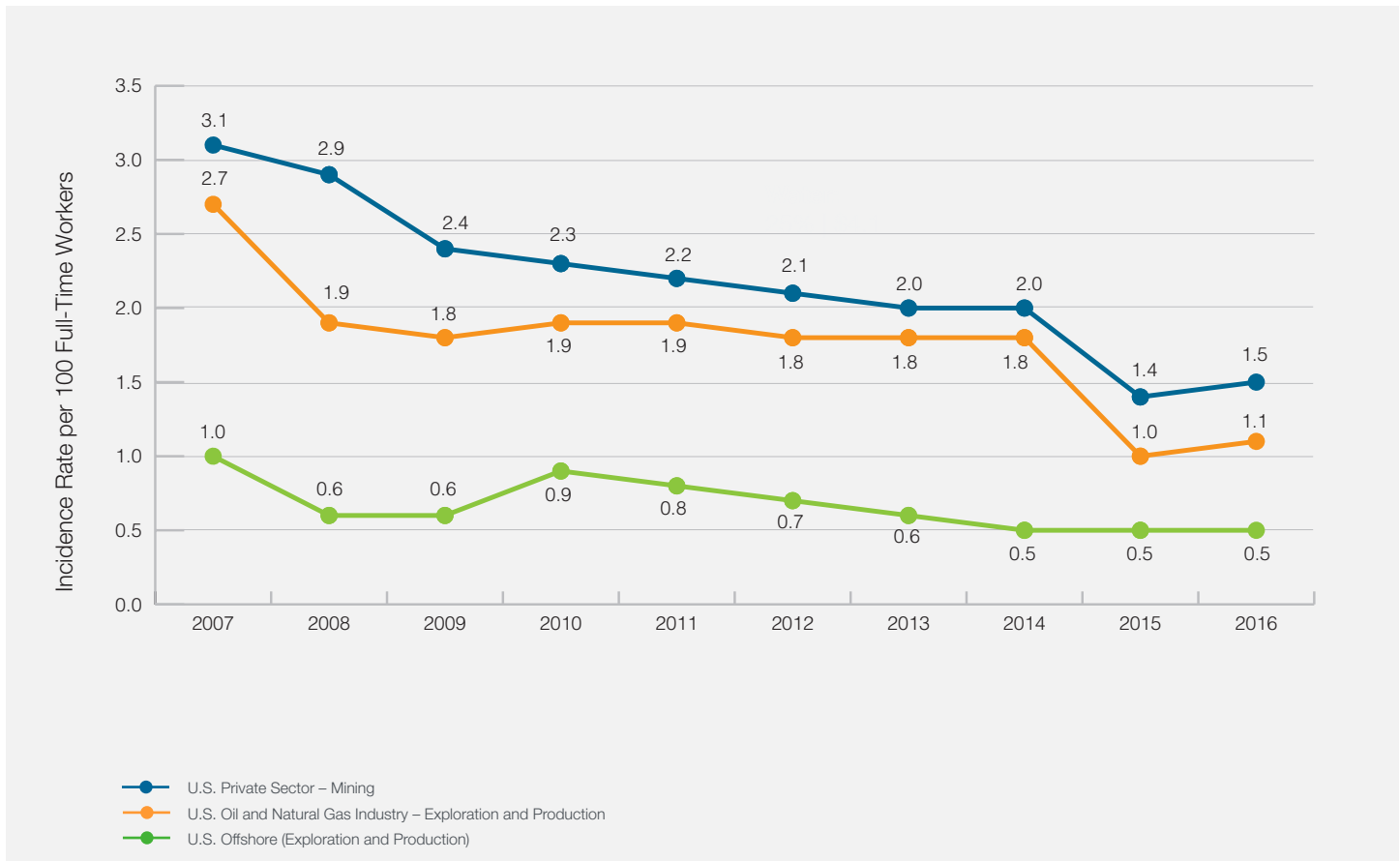
Figure 2 Exploration and Production vs. Mining (2007-2016)
